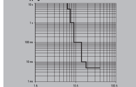
Tripping characteristic normal – AMG ELM-6F
