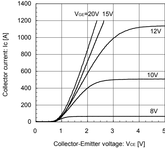
[INVERTER]
